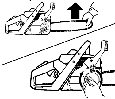
TIGHTEN
