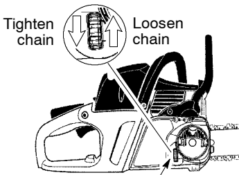
Adjusting Wheel
