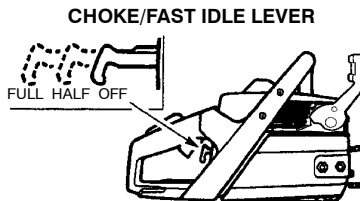
CHOKE/FAST IDLE LEVER
