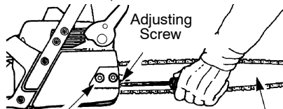
Chain Brake Nuts Guide Bar Adjusting Screw - 1/4 Turn
