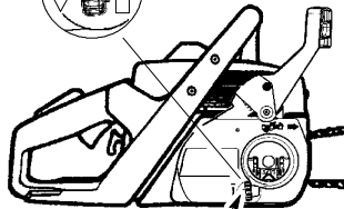
Adjusting Wheel
