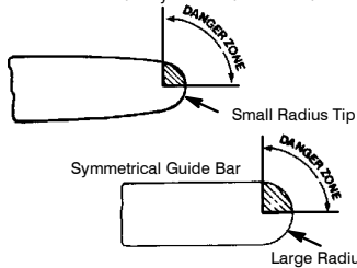
Reduced Kickback Symmetrical Guide Bar
