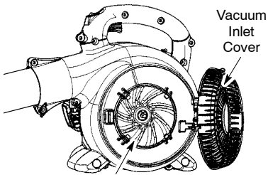
Vacuum Inlet
